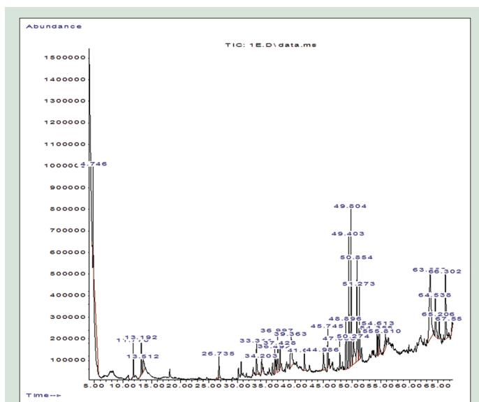
Figure 2: Gas chromatography–mass spectrometry chromatogram of ethanol extract of Helichrysum petiolare leaves
